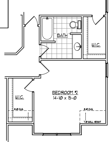
BEDROOM #2 OPTION
